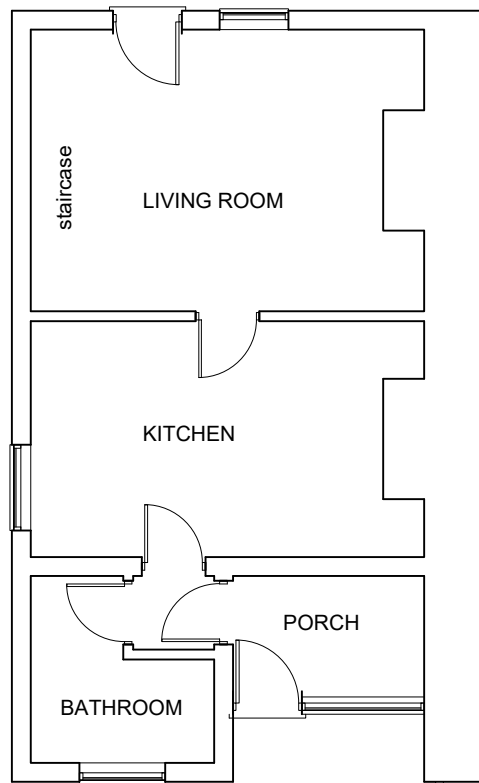
GROUND FLOOR PLAN No. 7
